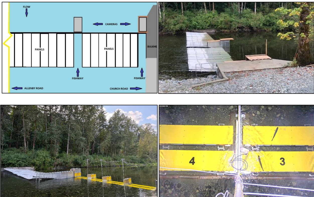
Figure 7: Traditional two-passage counting fence design used since 2019 (top) compared to the low-flow design with four open passageways and overhead camera views (bottom).
