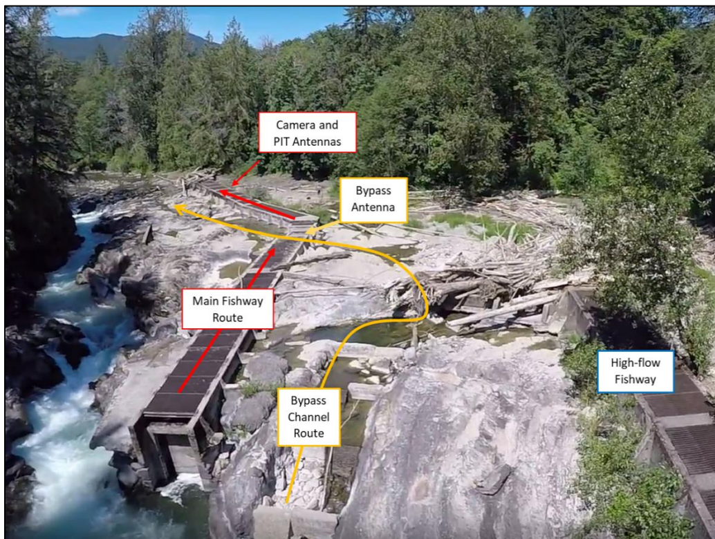
Figure 9: Skutz Fishways, bypass channel, migration routes, and monitoring equipment.
