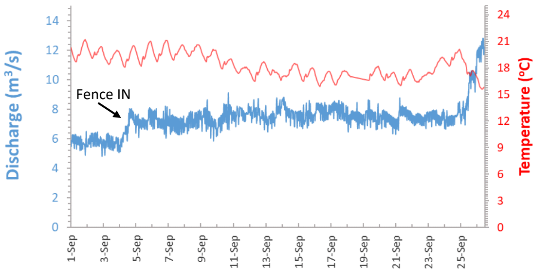
Figure 2: Discharge (m 3 /s) and Temperature (°C) at Water Survey of Canada Station 08HA011, Cowichan River in Duncan. Discharge levels when the salmon counting fence was installed are indicated.
